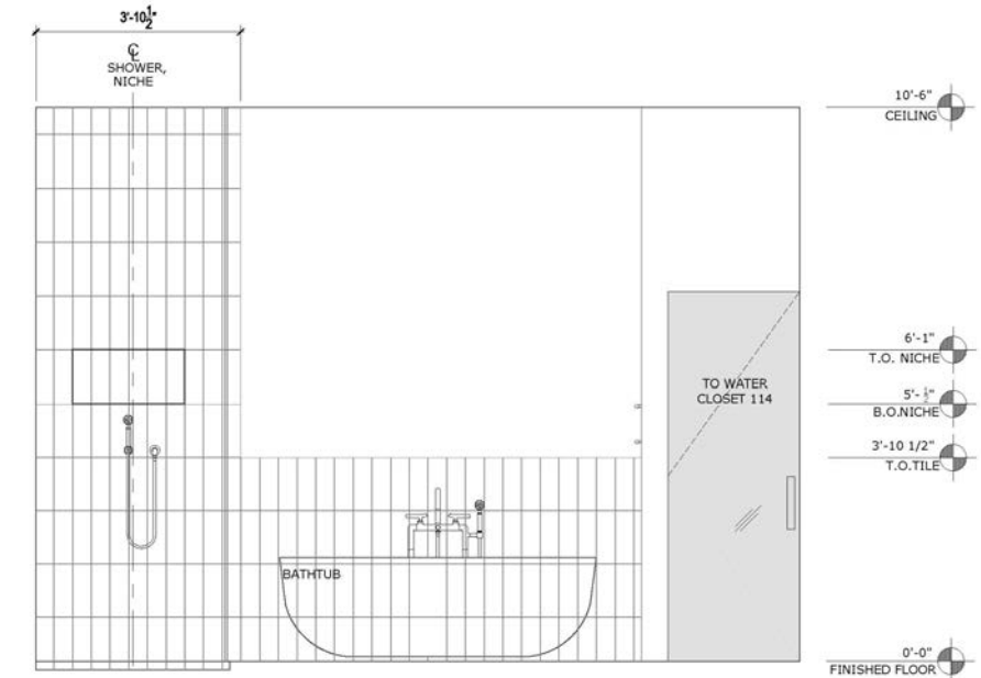
4 WEST ELEVATION: NICHE AT 2'-1 1/2" X 1'-0" SCALE: 1/2" = 1'-0"
