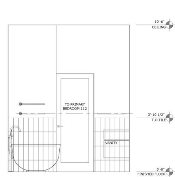
1 NORTH ELEVATION SCALE: 1/2" = 1'-0"
