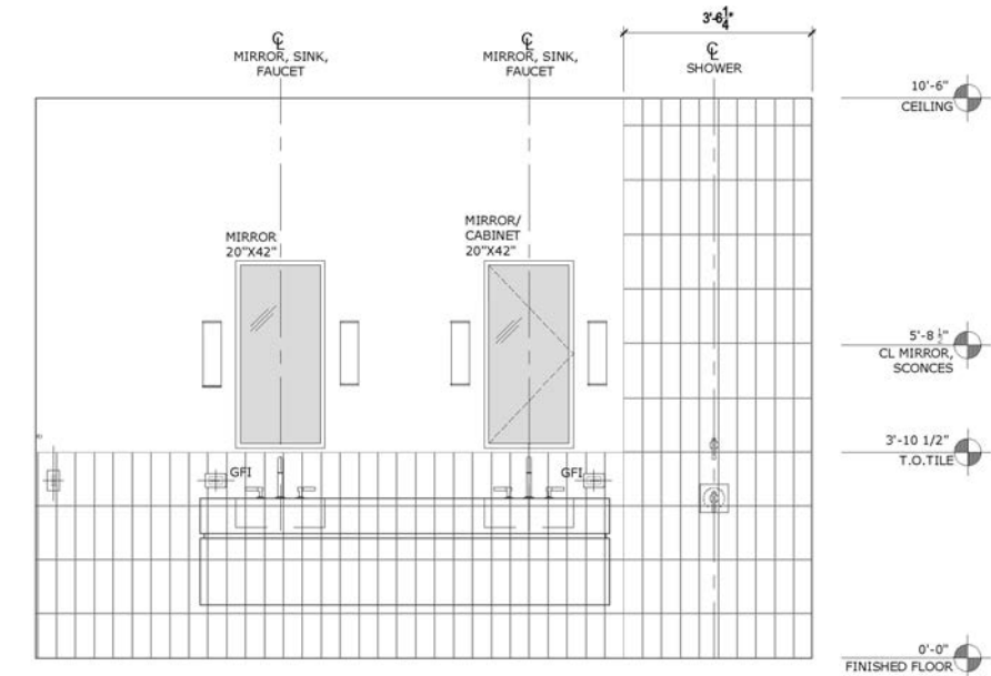
2 EAST ELEVATION SCALE: 1/2" = 1'-0"
